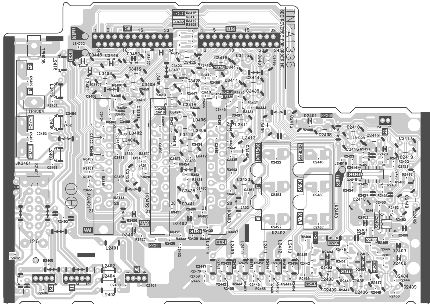
H-BOARD TNPA1336
