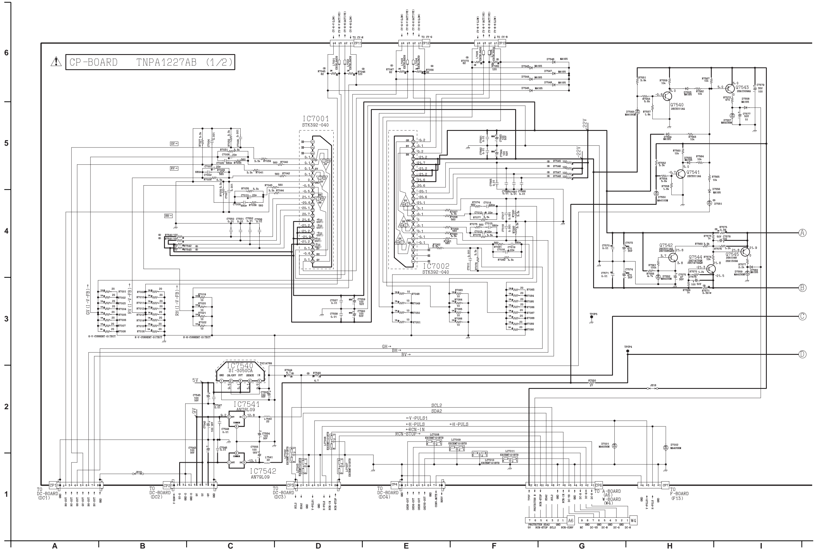
DC-BOARD/CP-BOARD
