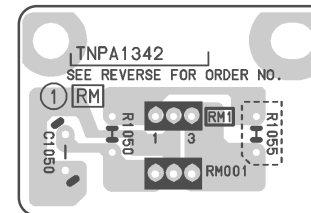
RM-BOARD TNPA1342
