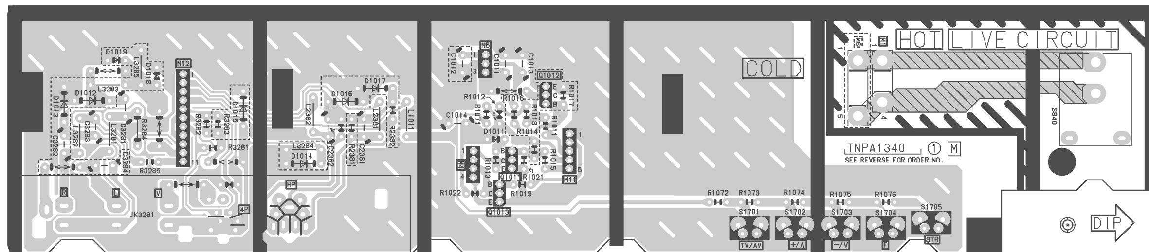
M-BOARD TNPA1340
