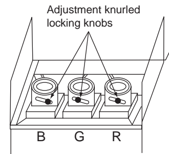
Optical lens focus adjustment
