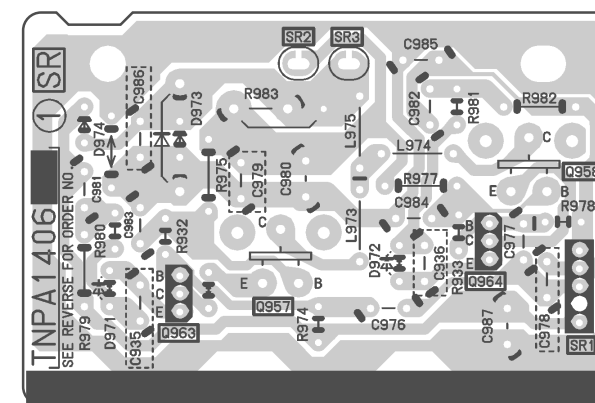
SR-BOARD TNPA1406
