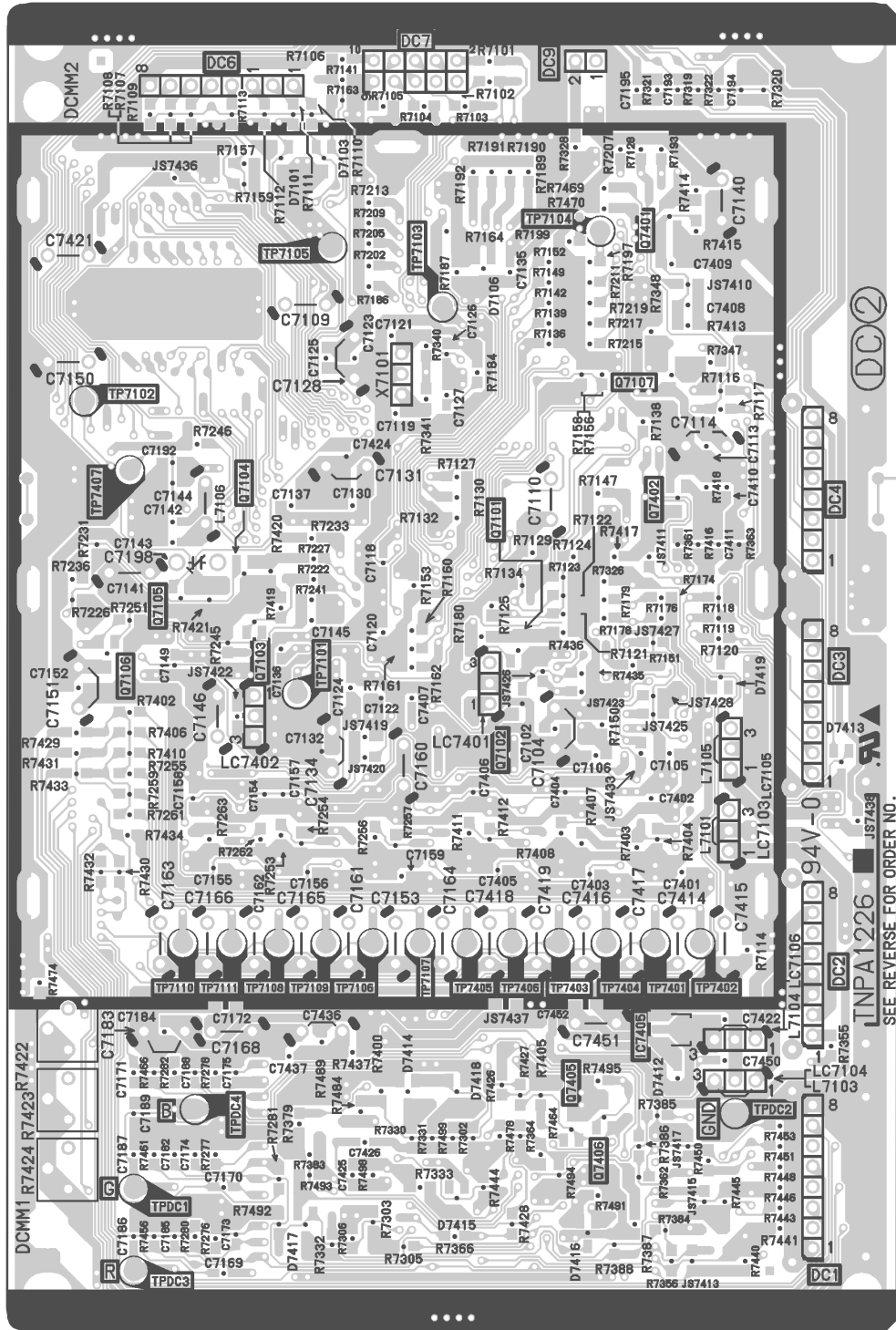
6 DC-BOARD (FOIL SIDE) TNPA1226AB
