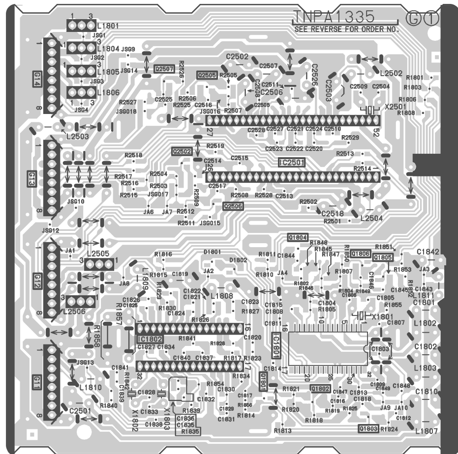
G-BOARD TNPA1335
